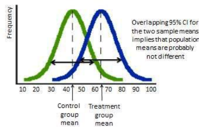
Figure 15.2. Student's t-test
