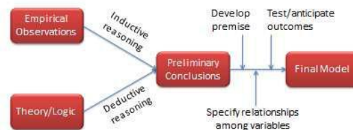
Figure 2.3. The model-building process
