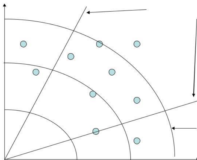
Figure 5.1. Internal and external validity
