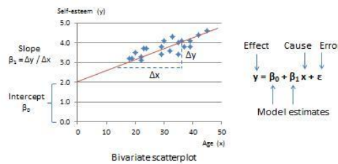
Figure 15.1. Two-variable linear model
