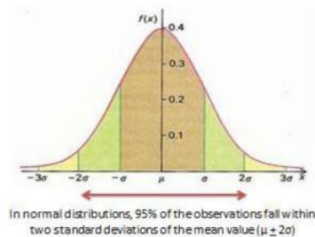
Figure 14.2. Normal distribution
