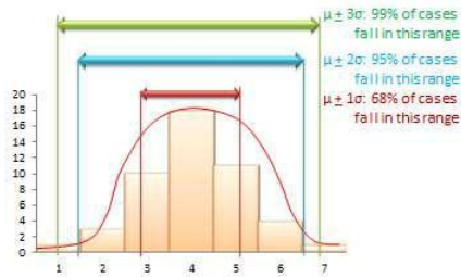
Figure 8.4. The 68-95-99 percent rule for confidence interval
