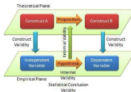
Figure 5.2. Different Types of Validity in Scientific Research
