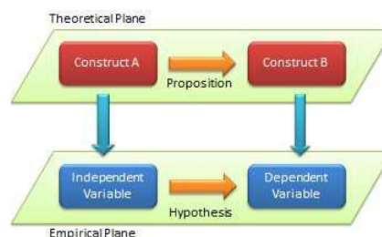
Figure 4.1. Distinction between theoretical and empirical concepts
