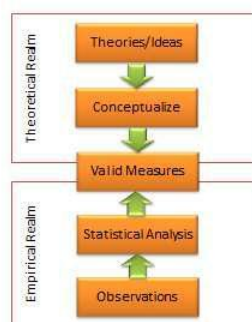
Figure 7.2. Two approaches of validity assessment
