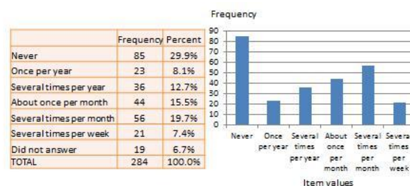
Figure 14.1. Frequency distribution of religiosity
