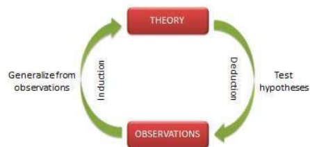
Figure 1.1. The Cycle of Research
