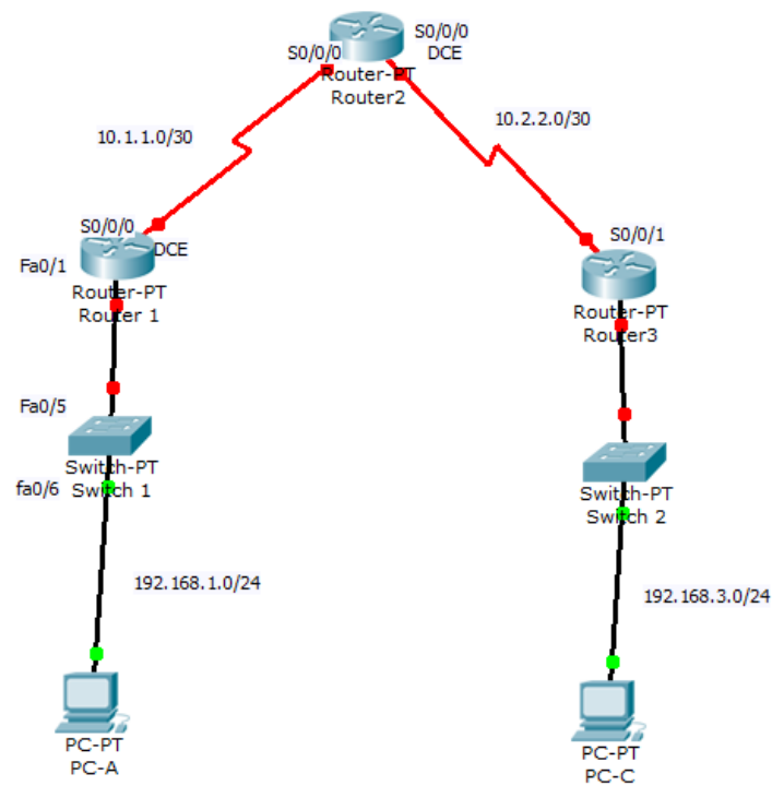
Fig 13: Lab 2 Topology
