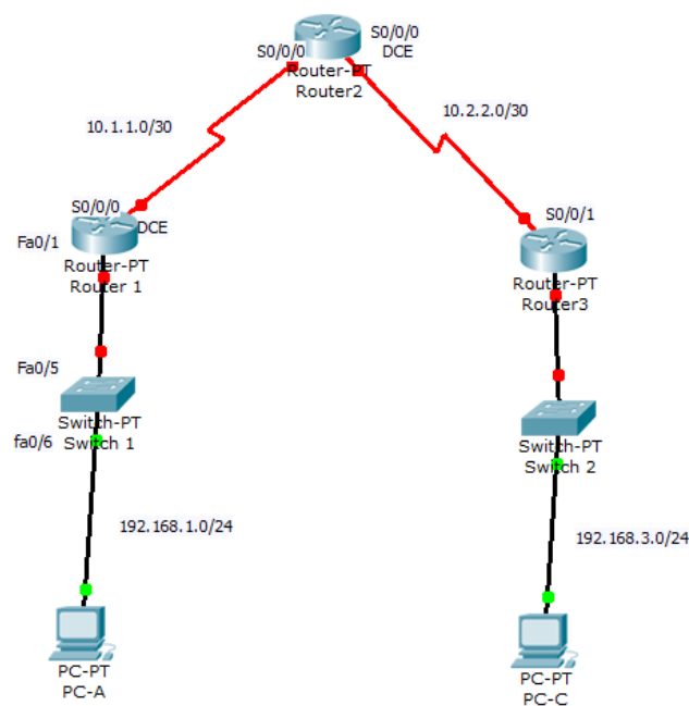
Fig 14: Lab 3 Topology
