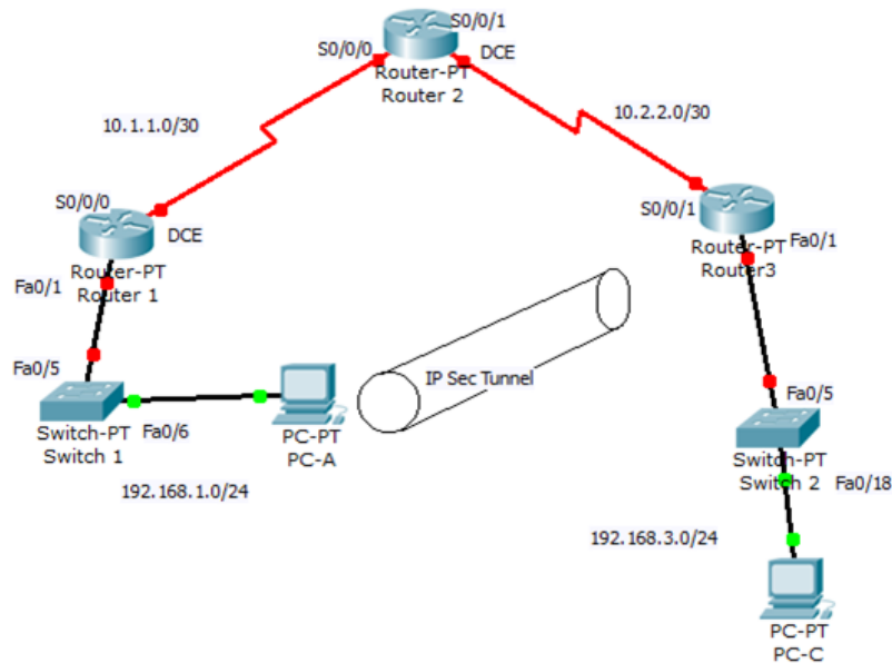
Fig 15: Lab 4 Topology
