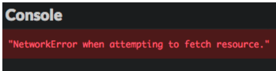
Execution result
