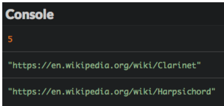
Expected result
