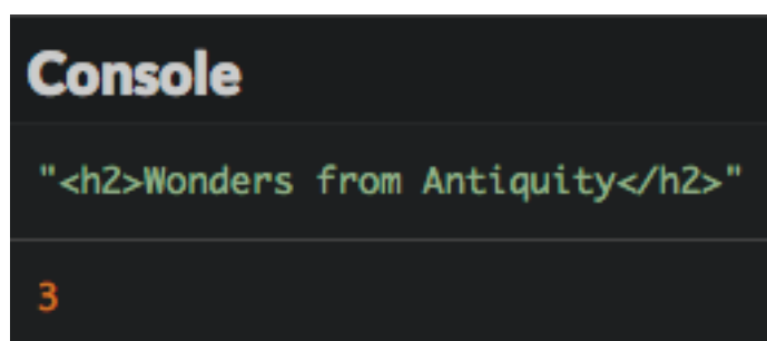
Execution result
