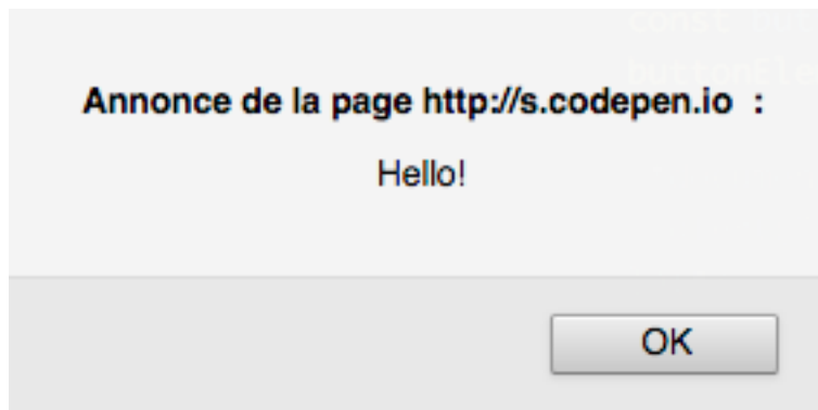
Execution result
