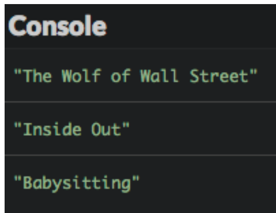
Execution result
