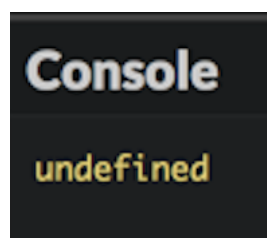
Execution result
