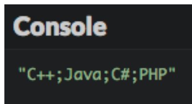
Execution result
