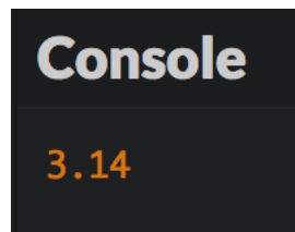
Execution result
