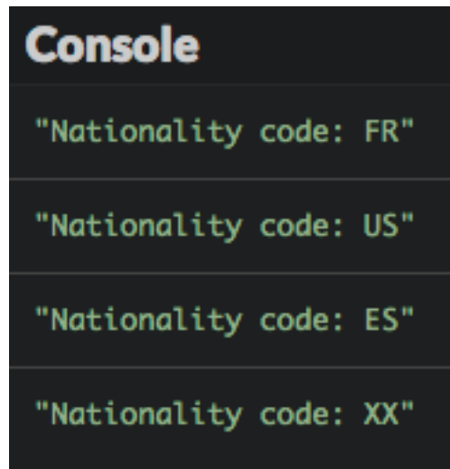
Execution result
