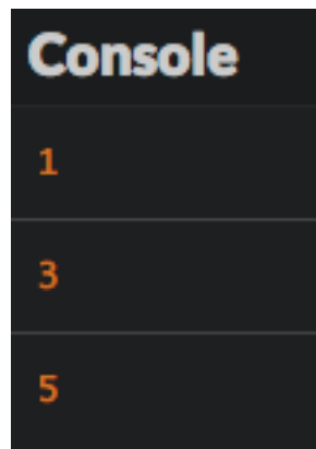
Execution result
