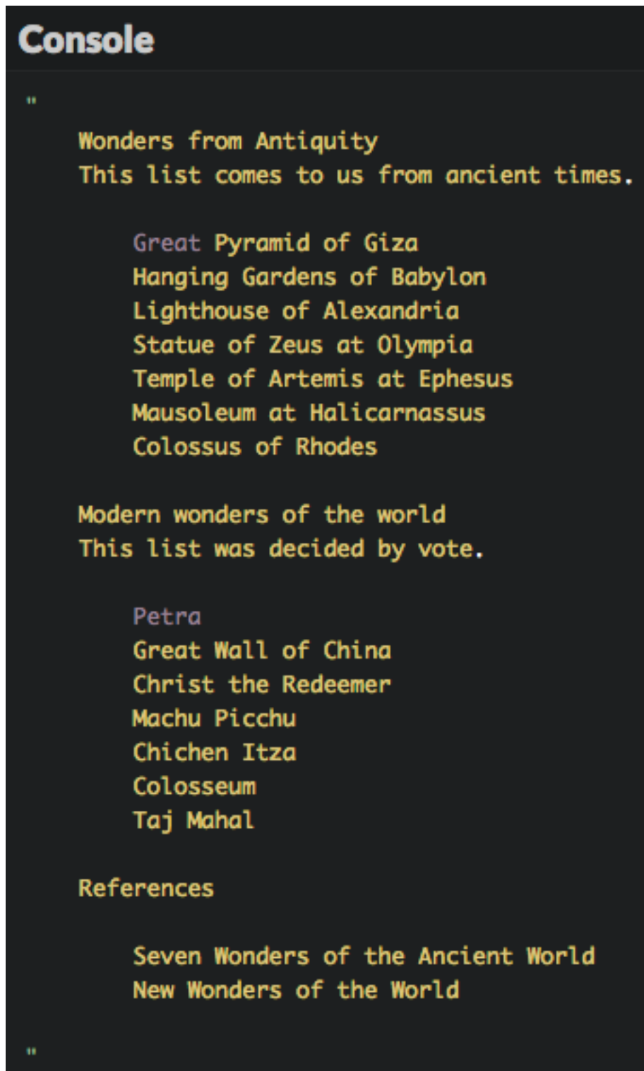
Execution result
