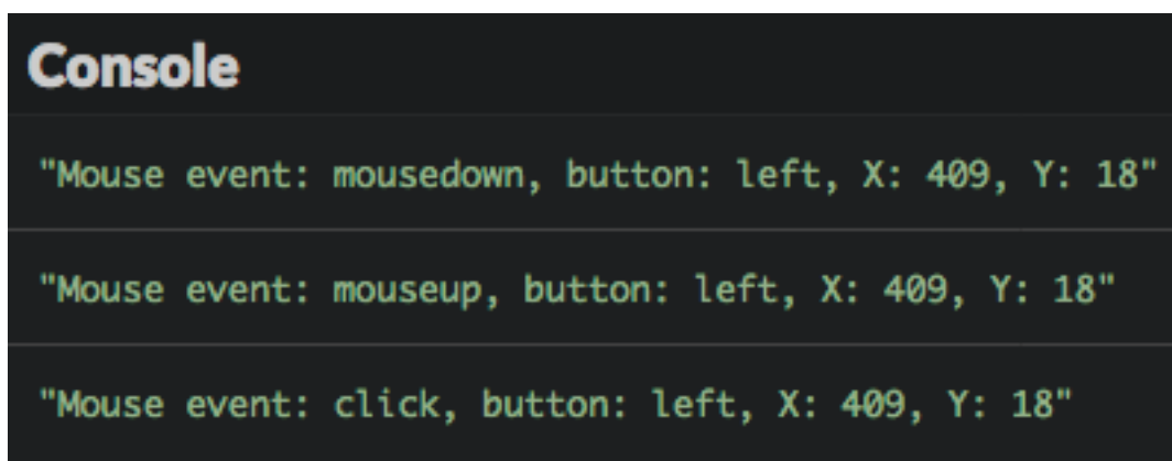
Execution result
