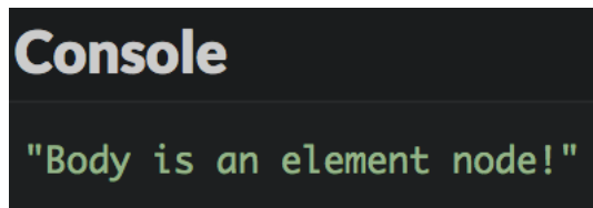
Execution result
