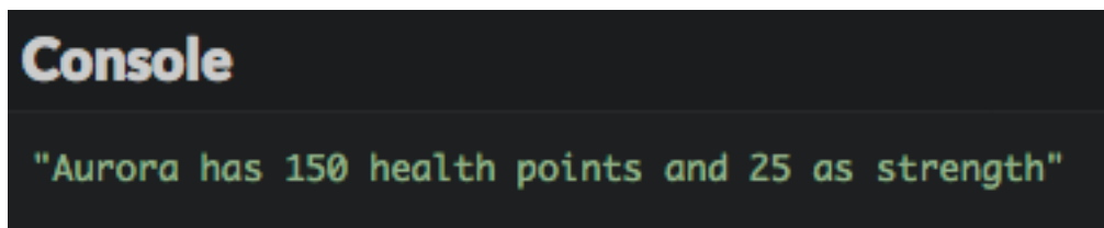
Execution result
