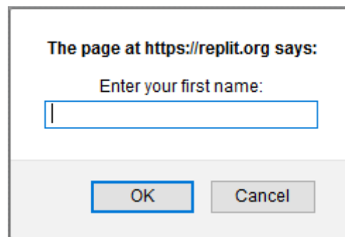
Execution result
