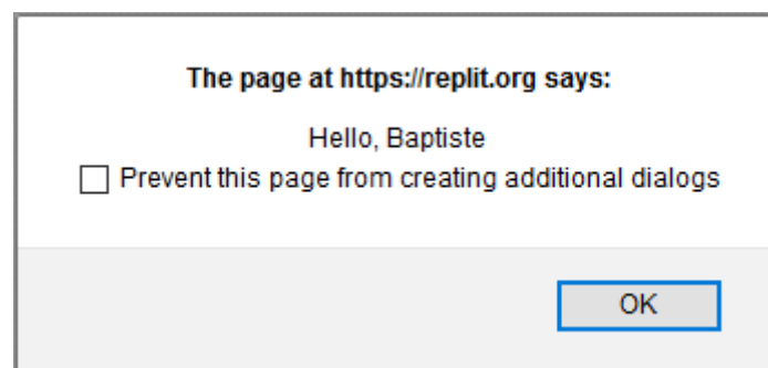
Execution result
