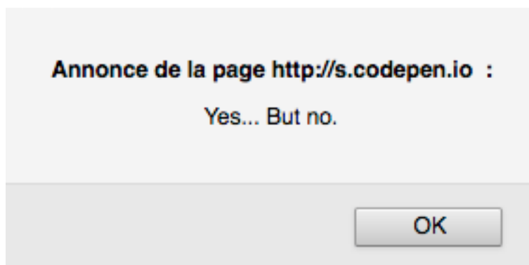
Execution result
