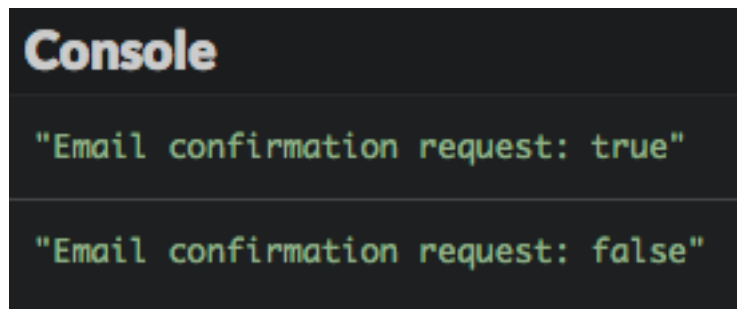
Execution result
