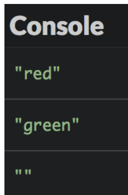
Execution result
