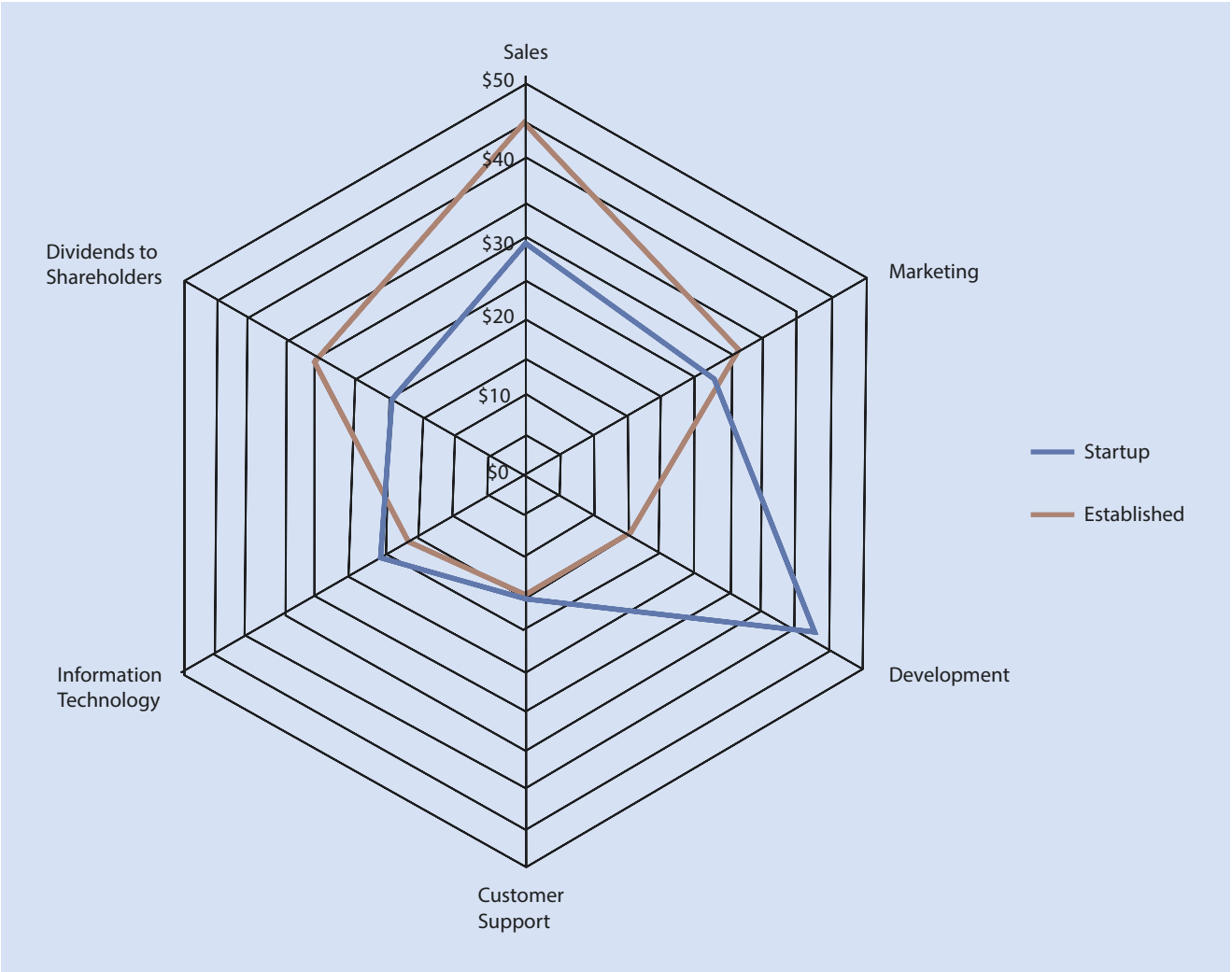
Fig. 14.7 Radar chart
