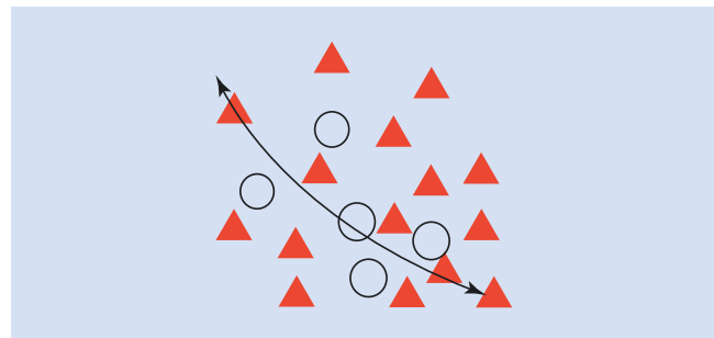
Fig. 9.11 Regression
