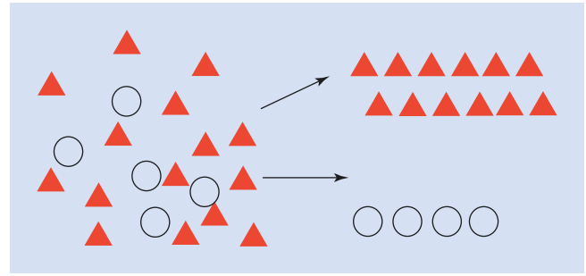
Fig. 9.5 Classification
