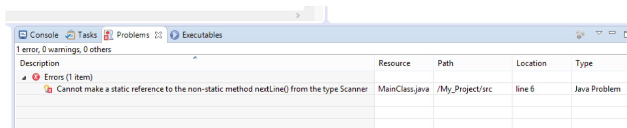
Figure 21: Error
