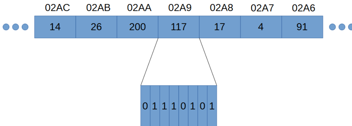
Figure 35: RAM
