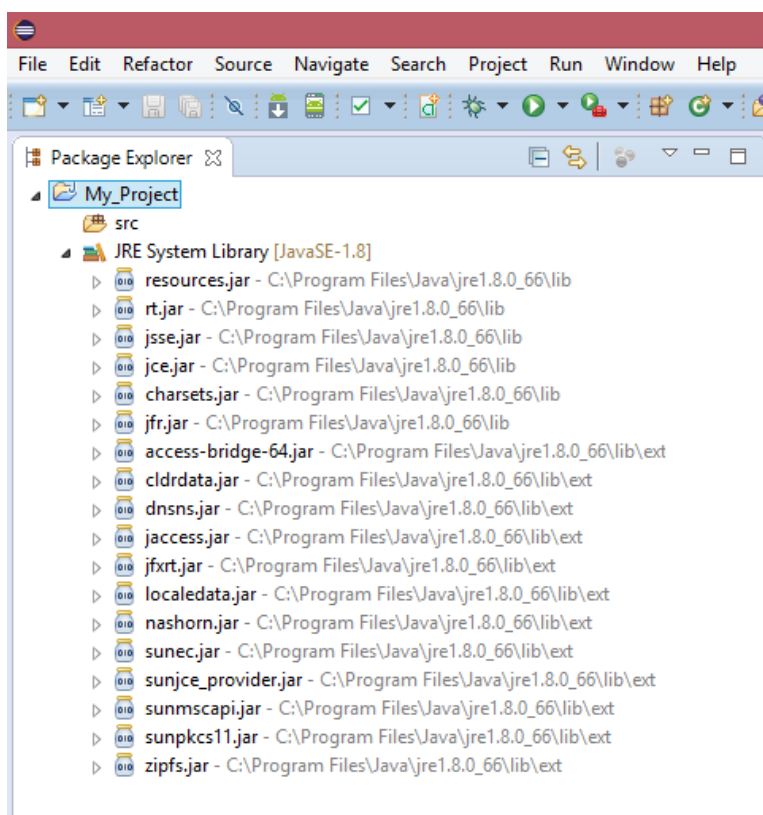
Figure 11: Package Explorer
