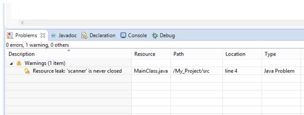
Figure 20: Warning
