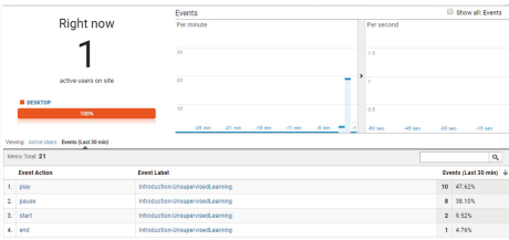
Fig. 7. Analytic dashboard
