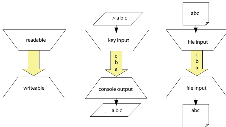
Figure 2.8 Streams can be of two types: readable streams, which access data, and writeable streams, which write data.
