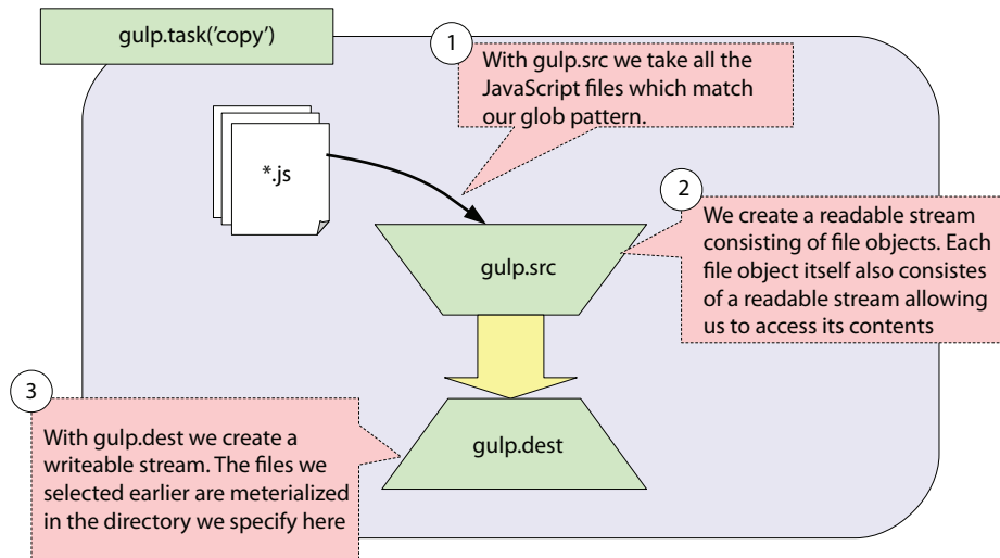
Figure 2.9 A basic Gulp task working with gulp.src and gulp.dest . You read files from one place and pipe their contents to a destination.
