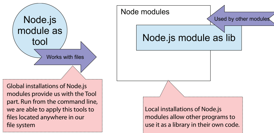
Figure 2.3 The two ways a Node.js module can be installed. If you install a module globally, it just provides its functionality as an executable from the command line, working with the files you want to change. It becomes a tool. Installed locally, you can use the same functionality but in your own programs.
