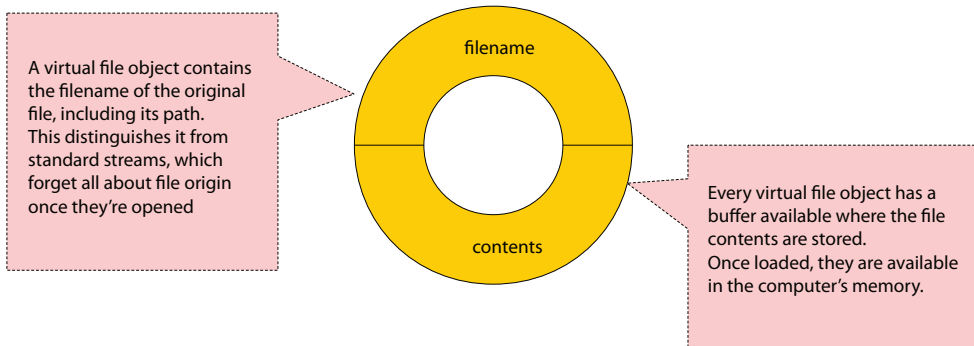
Figure 2.11 The symbol of a virtual file object. A virtual file consists mainly of two parts: data about the file's path and name, as well as a buffer containing the original contents. Both types of information are available in the computer's memory.
