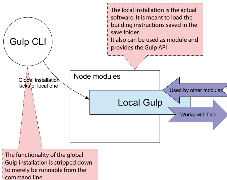
Figure 2.4 The global installation of Gulp is the Gulp CLI. Its purpose is to check the availability of a local installation, which it starts on call. The local Gulp is located in the local node_modules folder of a JavaScript project. It contains all the necessary runtime functions and provides an API for build files (Gulfiles).
