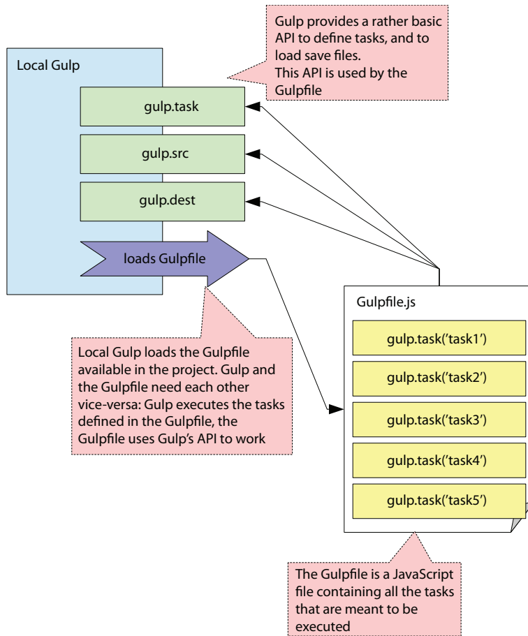
Figure 2.6 The local Gulp installation interplays with the Gulpfile. It loads the Gulpfile available in the project and executes the available tasks, as instructed by the command-line interface. It also provides the Gulpfile with a basic API, which is needed to create and define tasks.
