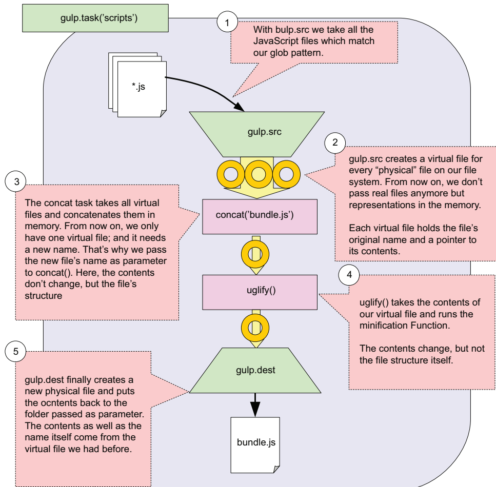
Figure 2.12 Streams applied to the virtual file system and Gulp. With gulp.src you select a sequence of files, promote them to the virtual file system as file objects, and access their contents for a series of transformation processes provided by the Gulp plugins.
