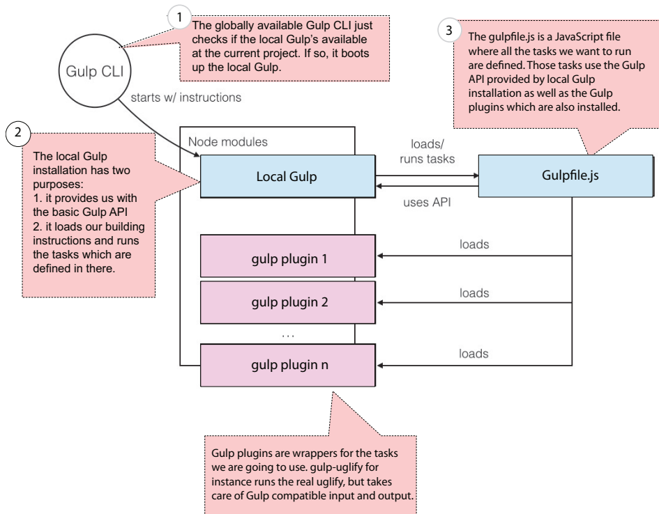
Figure 2.2 The Gulp CLI starts the local Gulp installation with the parameters provided on the command line. The local installation takes the local Gulpfile, which in turn loads Gulp plugins and defines tasks using the Gulp API. Gulp itself runs and loads these tasks.
