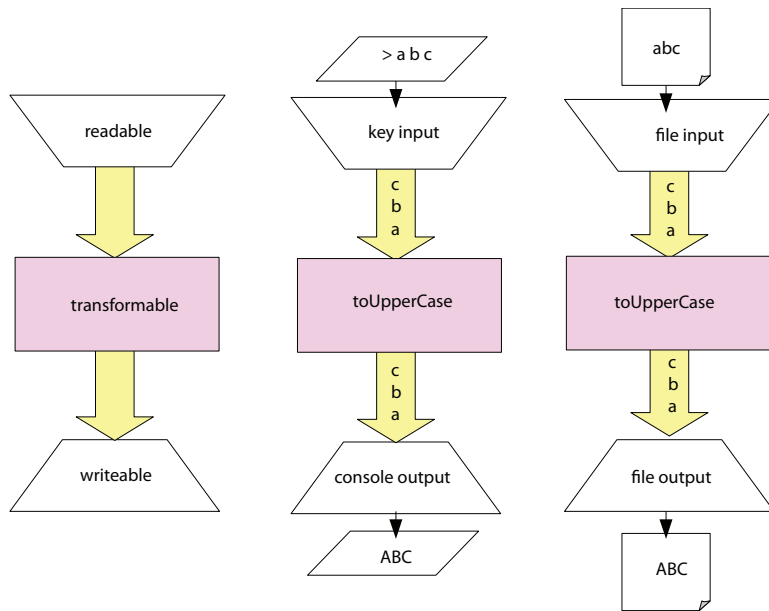
Figure 2.10 Streams are good not only for transferring data but also for modifying it.
