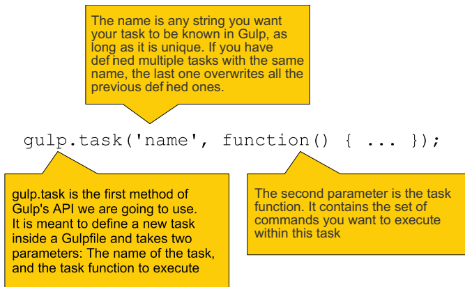
Figure 2.5 The signature of the gulp.task method
