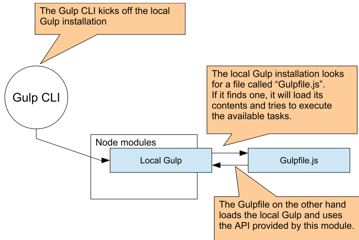
Figure 2.7 The global CLI kicks off the local Gulp. The local Gulp looks for a Gulpfile and loads its contents.
