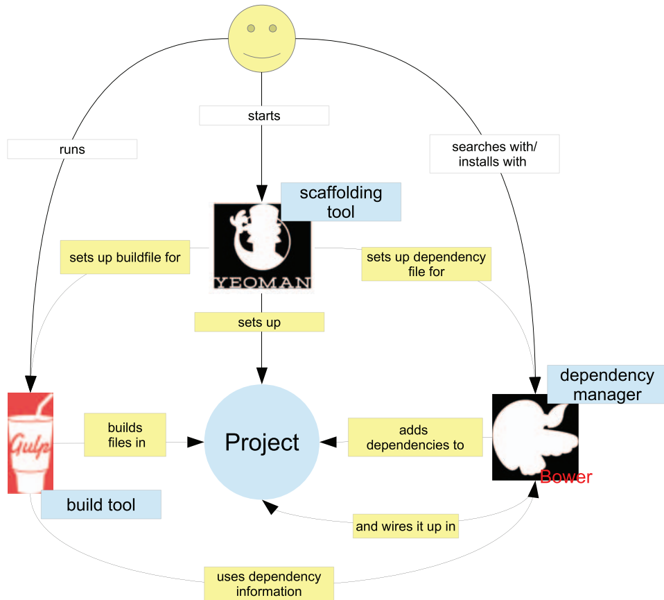
Figure 2.1 Your workflow setup from chapter 1
