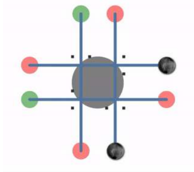
Figure 11.1.1: Four processes (blue lines) compete for one resource (grey circle), following a right-before-left policy. A deadlock occurs when all processes lock the resource simultaneously (black lines). The deadlock can be resolved by breaking the symmetry. ("Marble Machine" by Wikimedia Commons is licensed under CC BY-SA 4.0 )
