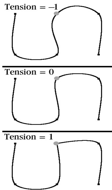
Figure 12.5 The effect of varying the tension parameter at a key frame on a 2D K-B spline curve
