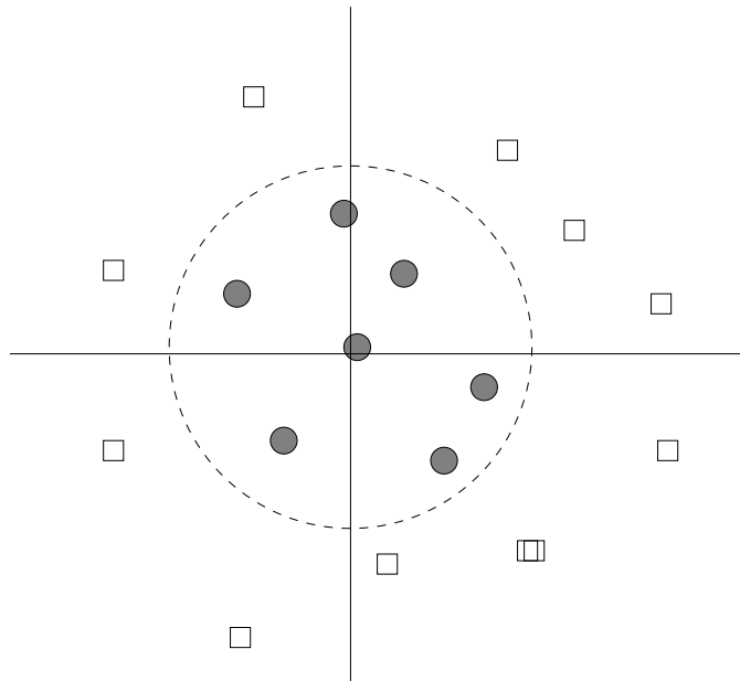
Figure 12.9: Transforming from rectangular to polar coordinates turns this training set into one with a separating hyperplane
