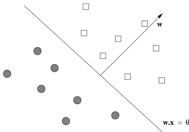
Figure 12.3: A perceptron divides a space by a hyperplane into two half-spaces
