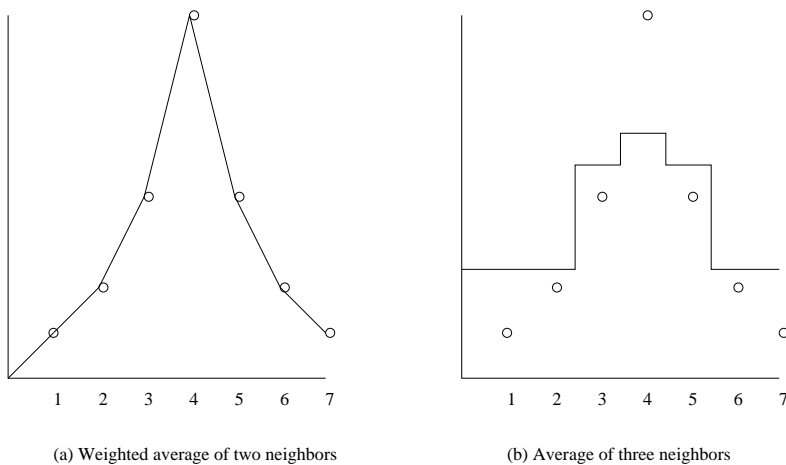
Figure 12.22: Results of applying the last two rules in Example 12.11
