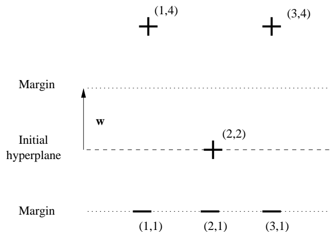
Figure 12.17: Six points for a gradient-descent example
