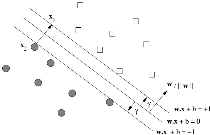
Figure 12.14: Normalizing the weight vector for an SVM
