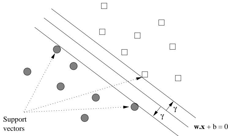
Figure 12.13: An SVM selects the hyperplane with the greatest possible margin \gamma between the hyperplane and the training points
