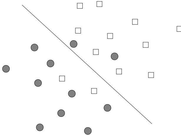
Figure 12.10: A training set may not allow the existence of any separating hyperplane
