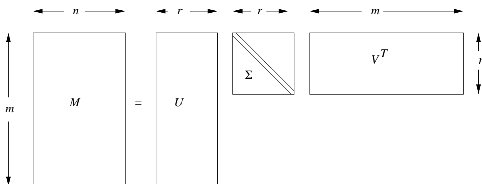
Figure 11.5: The form of a singular-value decomposition
