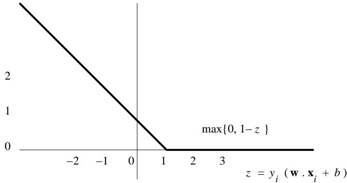
Figure 12.16: The hinge function decreases linearly for z \leq 1 and then remains 0
