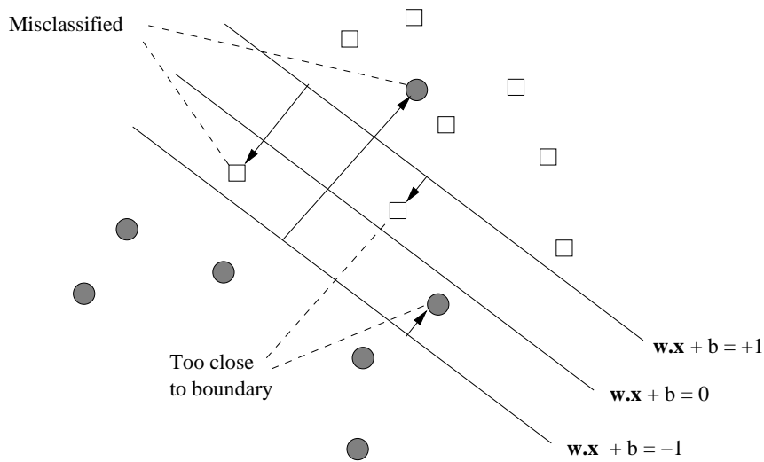
Figure 12.15: Points that are misclassified or are too close to the separating hyperplane incur a penalty; the amount of the penalty is proportional to the length of the arrow leading to that point
