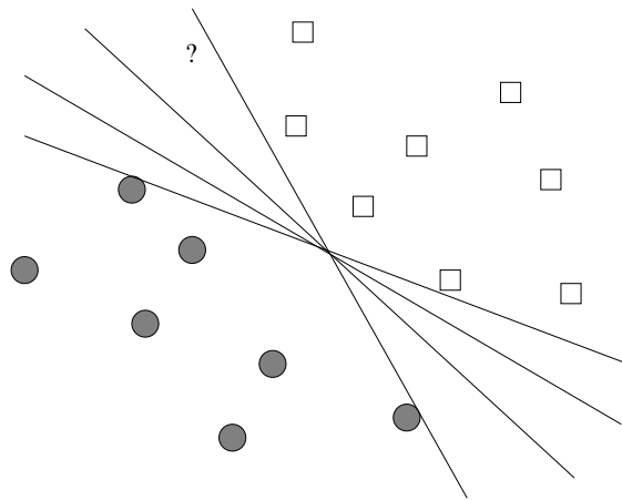
Figure 12.11: Generally, more than one hyperplane can separate the classes if they can be separated at all
