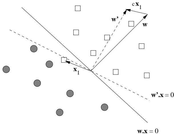
Figure 12.4: A misclassified point \mathbf{x}_1 moves the vector \mathbf{w}
