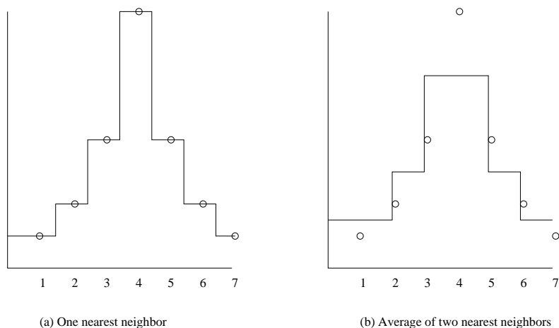
Figure 12.21: Results of applying the first two rules in Example 12.11
