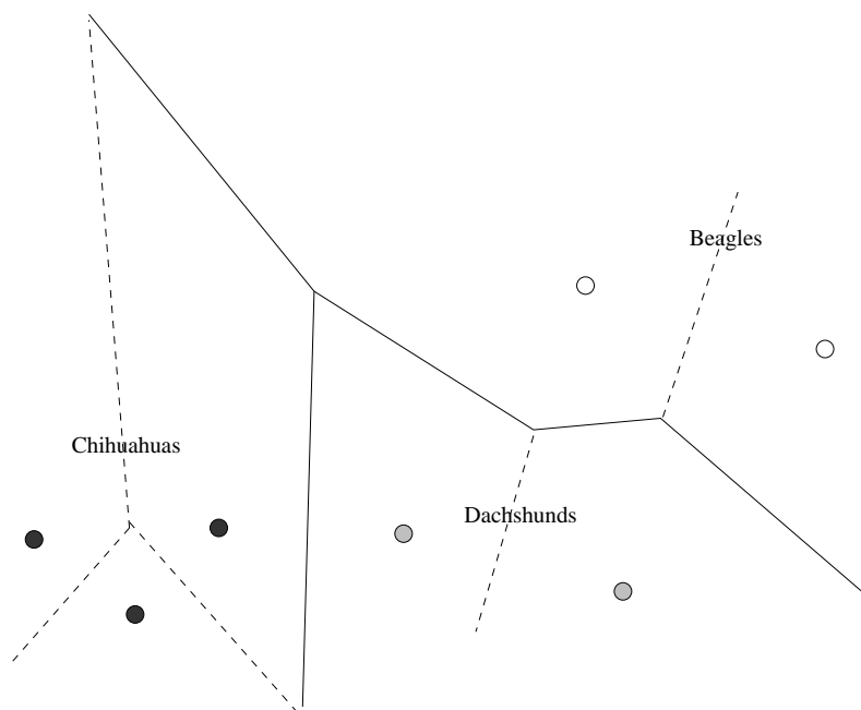
Figure 12.20: Voronoi diagram for the three breeds of dogs
