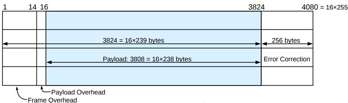
OTN Frame Format: 4080 columns × 4 rows
