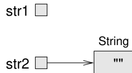
Figure 9.5: Memory diagram of null and empty string.
